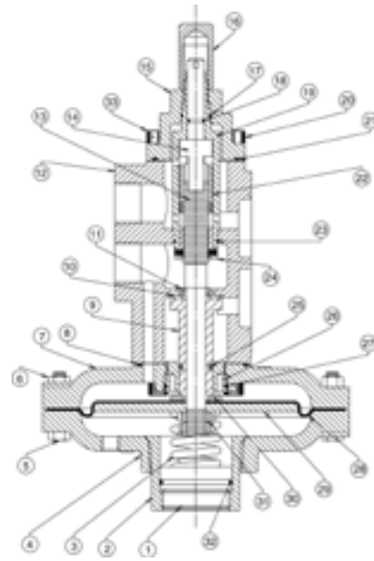
415 Control Valve
